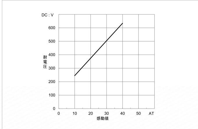
接点間耐圧
